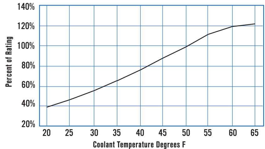
Derating Curve
