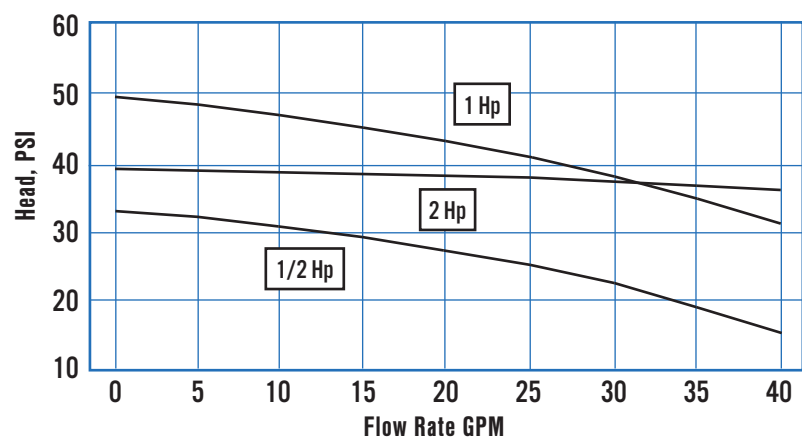
Pump Performance
