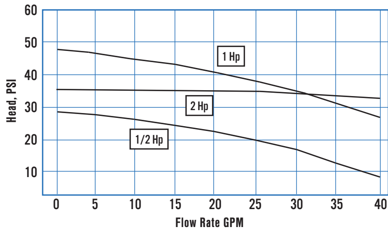
Pump Performance
