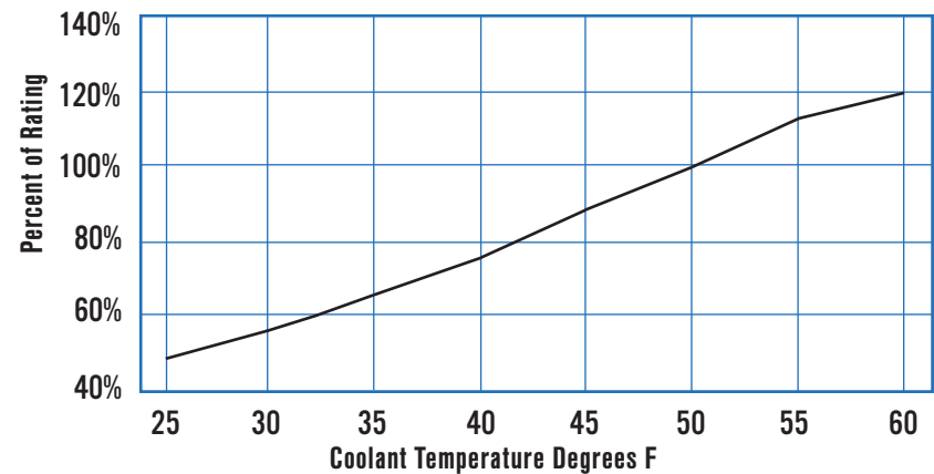
Derating Curve
