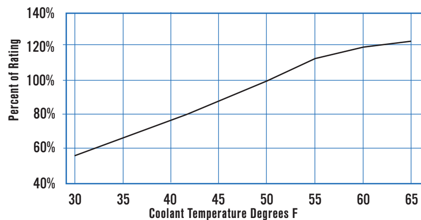
Derating Curve
