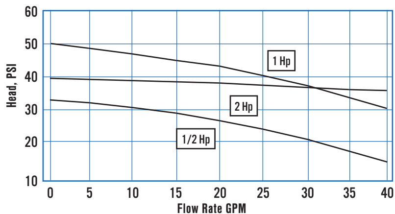
Pump Performance
