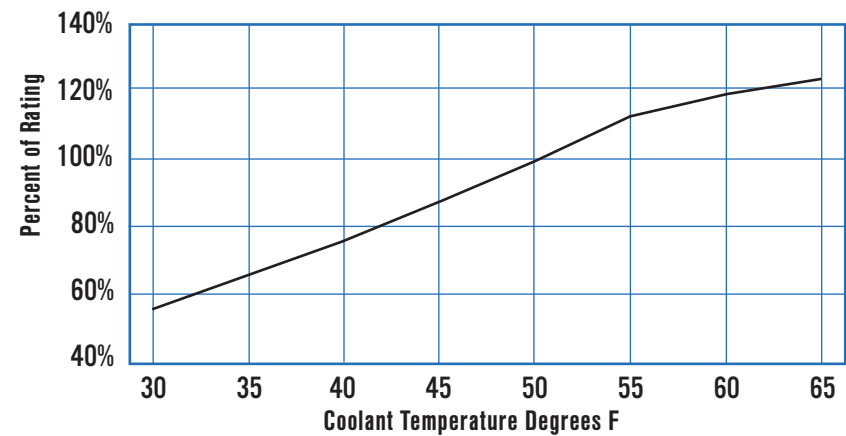
Chiller Section Derating Curve
