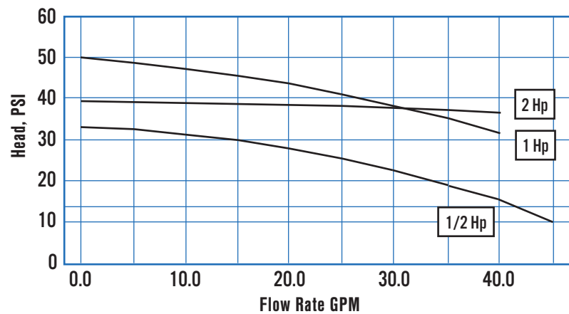
Pump Performance 1/2 and 1HP
